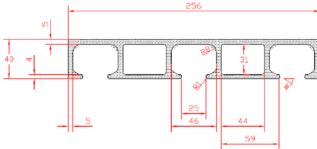
Figur 5: Geometrie Planke 256.40
